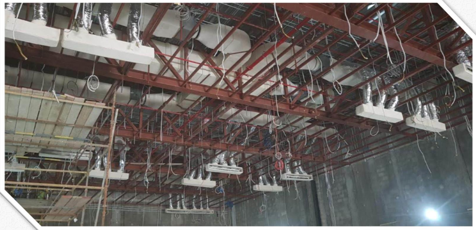
Over Ceiling MEP Works
