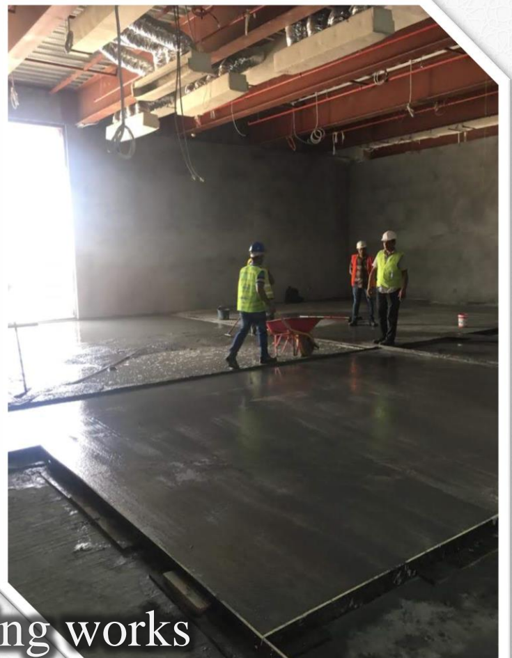
Concreteing works
